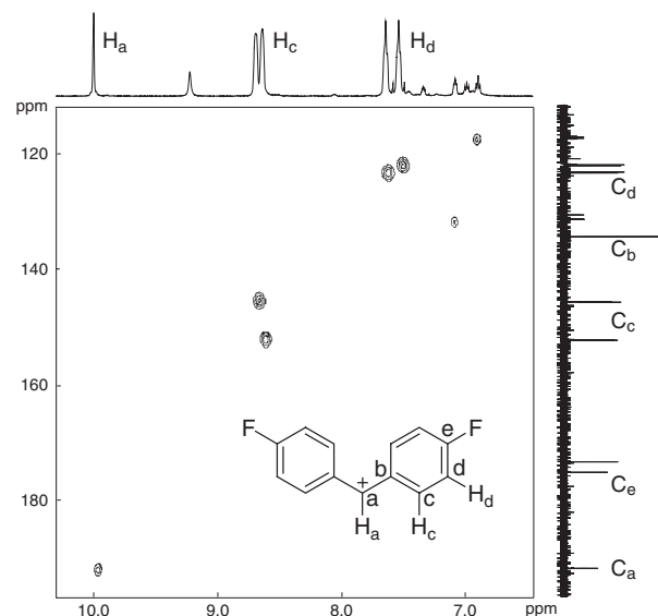
Figure 1. HMQC spectrum of diarylcarbenium ion 2k . NMR measurement was performed at -78^\circ\text{C} in \text{CD}_2\text{Cl}_2 with \text{CH}_2\text{Cl}_2 as an internal standard ( ^1\text{H} NMR: 600 MHz, ^{13}\text{C} NMR: 150 MHz).
